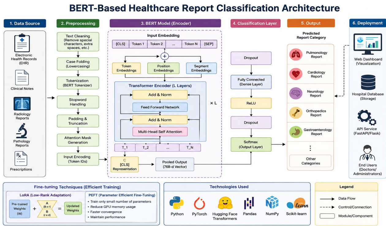
Fig 2: BERT Classification Pipeline
